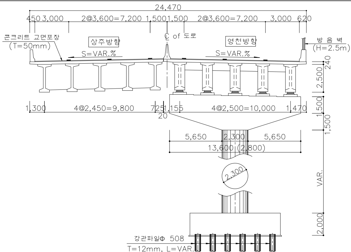
[횡단면도]
